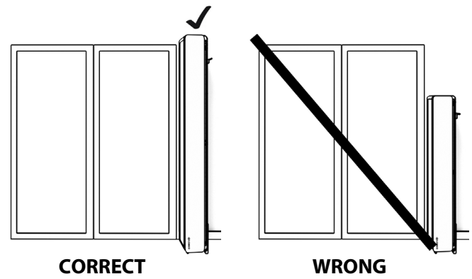
PIC. 5.2 VERTICAL INSTALLATION.
