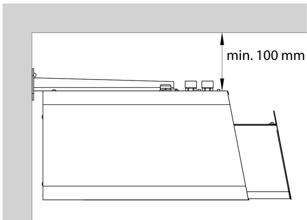
PIC. 6.1 MOUNTING WITH DEDICATED BRACKETS.
