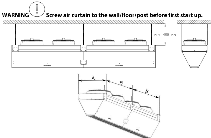
PIC. 8.1 HORIZONTAL INSTALATION
