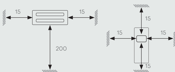
Internal split unit
