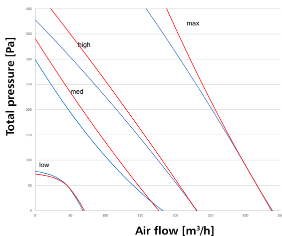
HRU-SlimAIR-300-H — SUPPLY — EXHAUST
