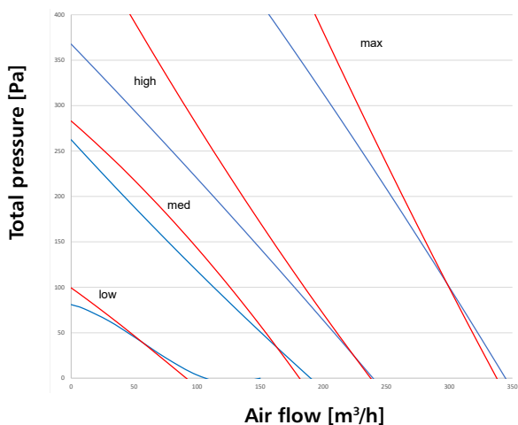
HRU-SlimAIR-300E-H — SUPPLY — EXHAUST
