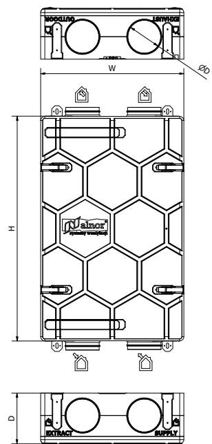
HRU-SlimAIR-L (only 250 and 300 models)
