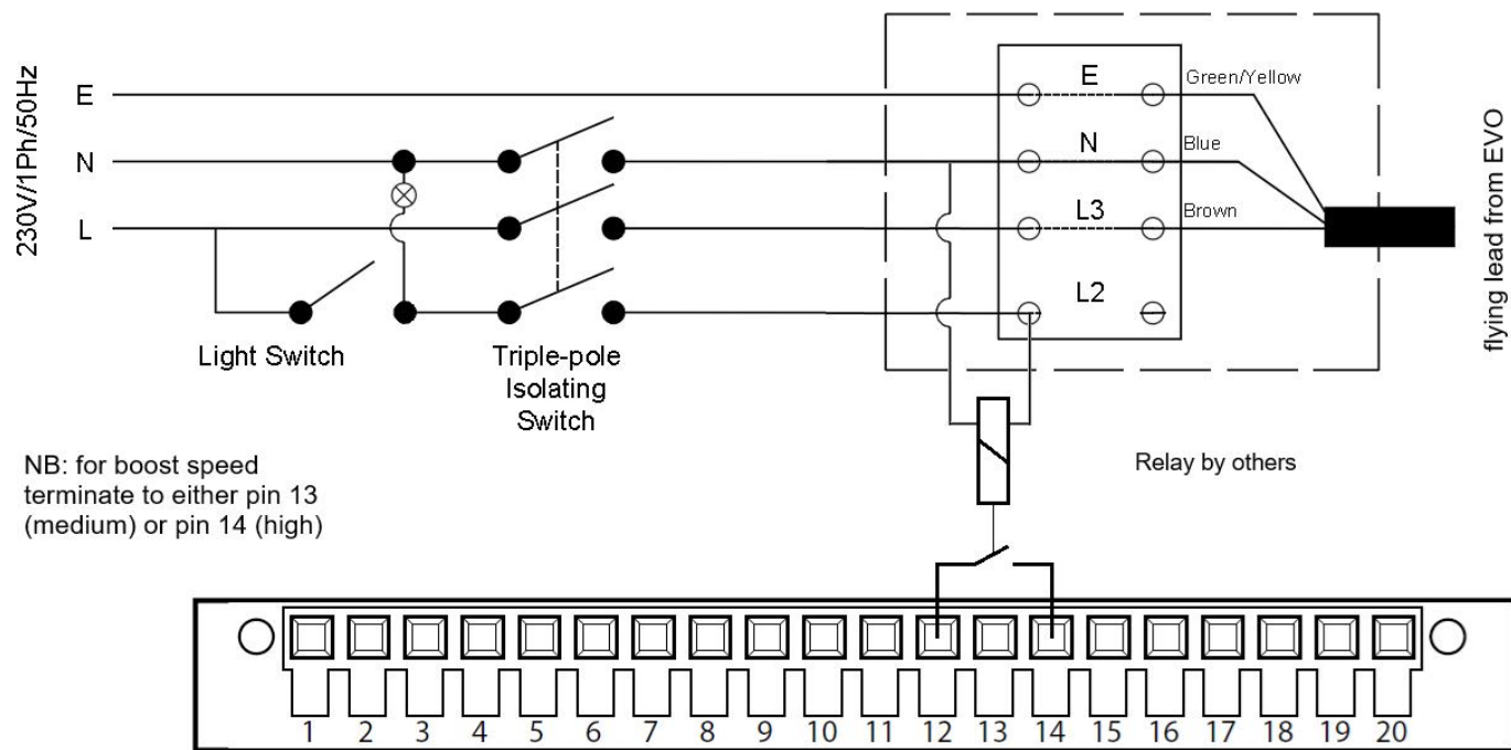
Integral control circuit board on EVO
